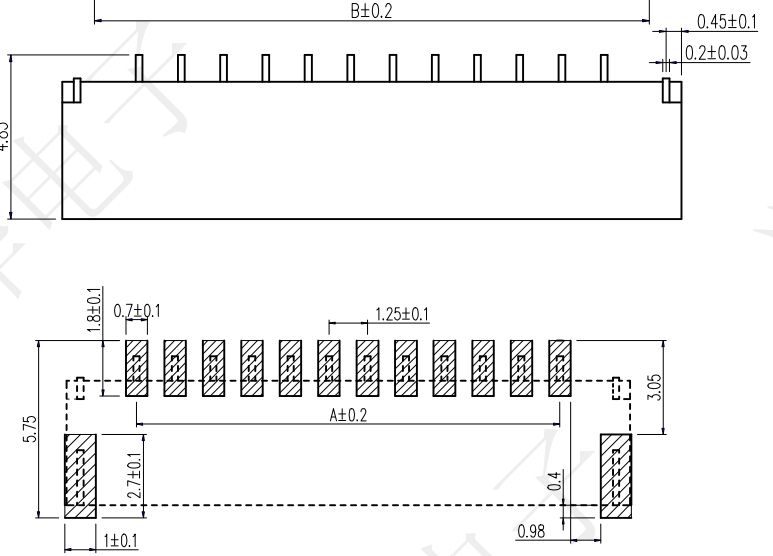
PCB LAYOUT
