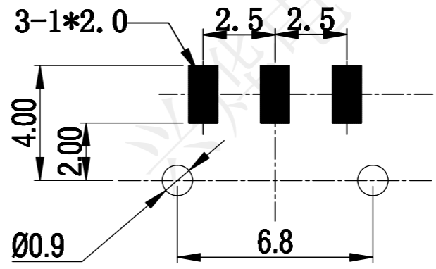
P. C. B LAYOUT DIMENSION
