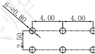
P.C.B LAYOUT DIMENSION TOP VIEW
