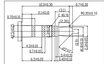
(φ2.50mm 4 POLE PLUG DETAIL DRAWING)
