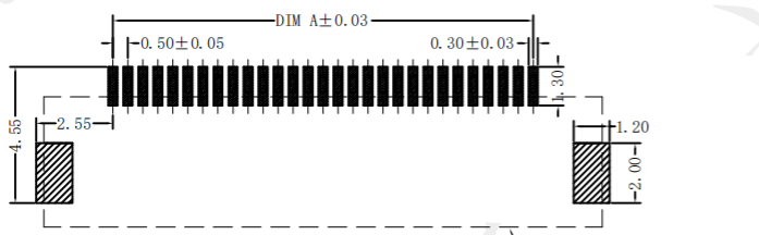
CONNECTOR POSITION
