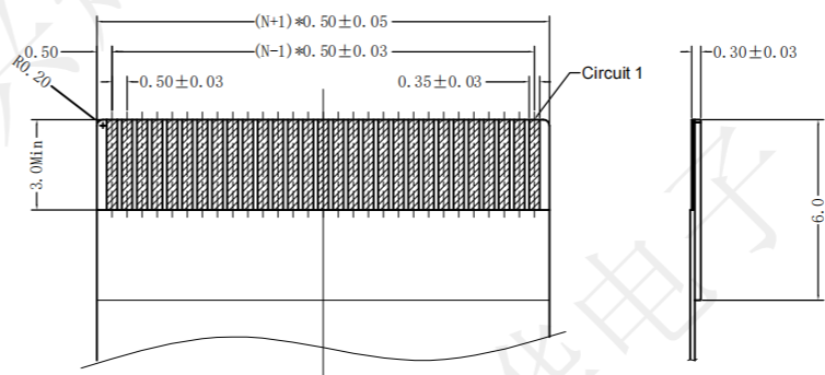
RECOMMENDED FPC/FC DIMENSION
