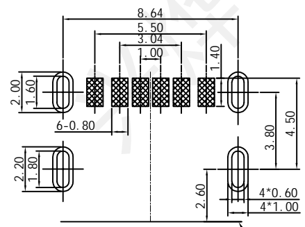
RECOMMENDED P.C.B. LAYOUT TOLERANCE UNSPECIFIED ±0.05mm
